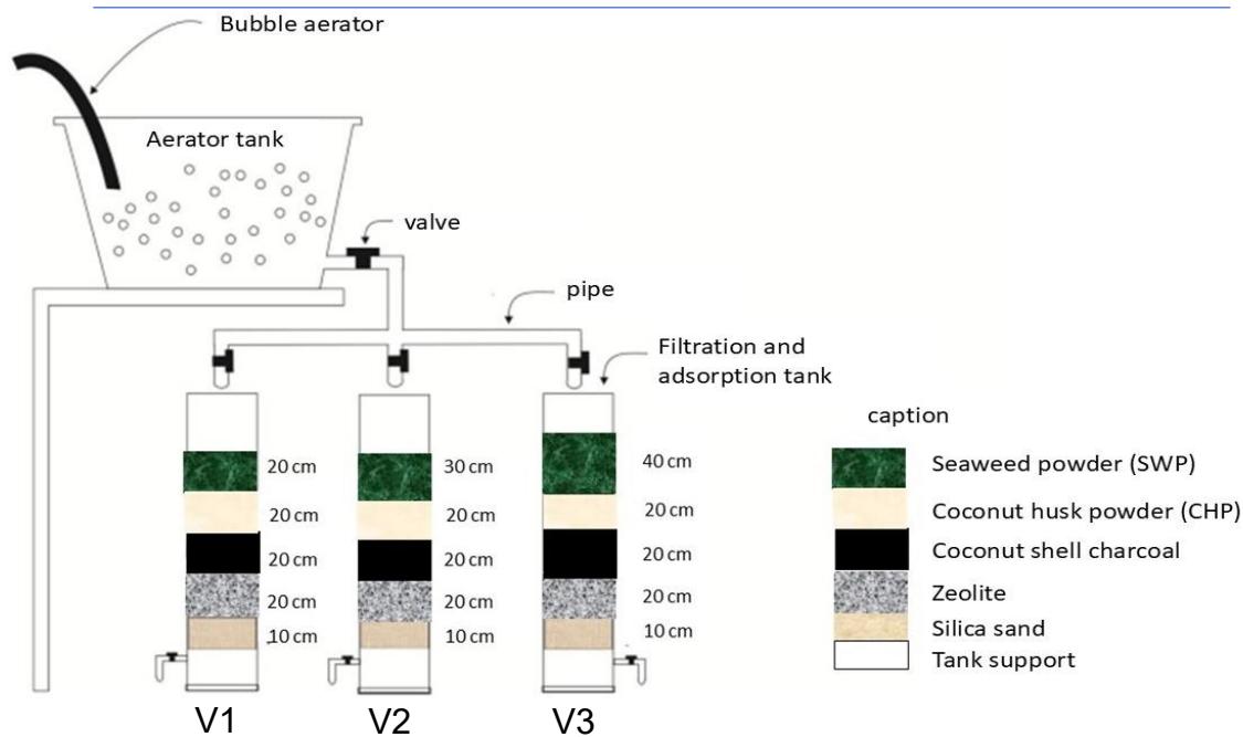
Figure 1. Filtration and adsorption tank model with combined SWP and CHP adsorbents
